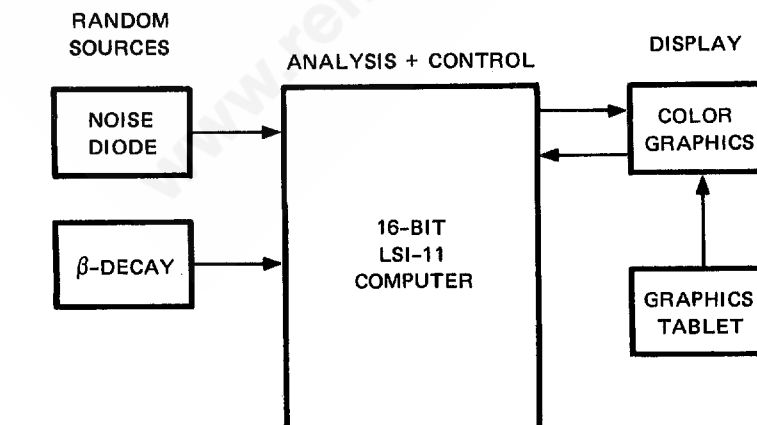
FIGURE 1 (U) BLOCK DIAGRAM OF COMPUTER-BASED RNG SYSTEM
